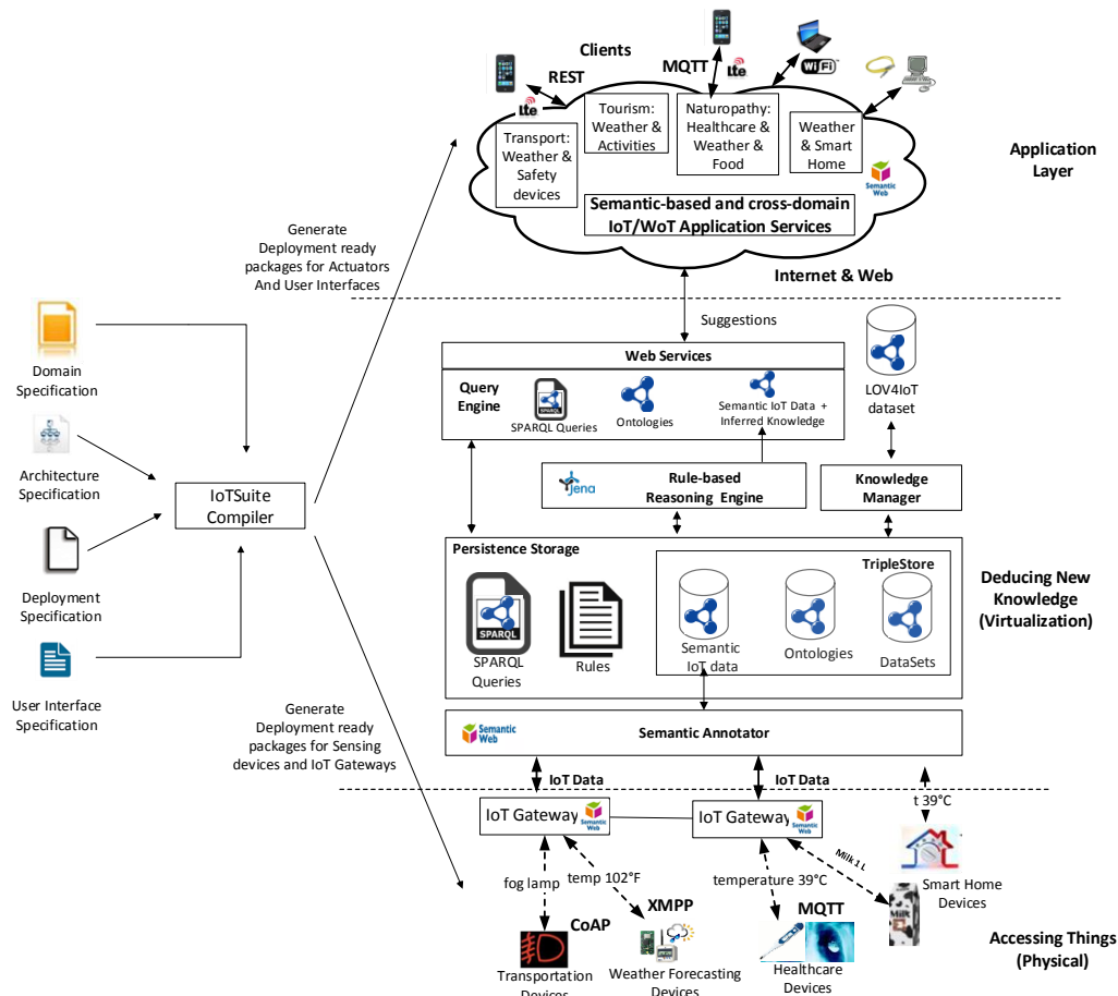
Figure 1: SWoTSuite architecture
