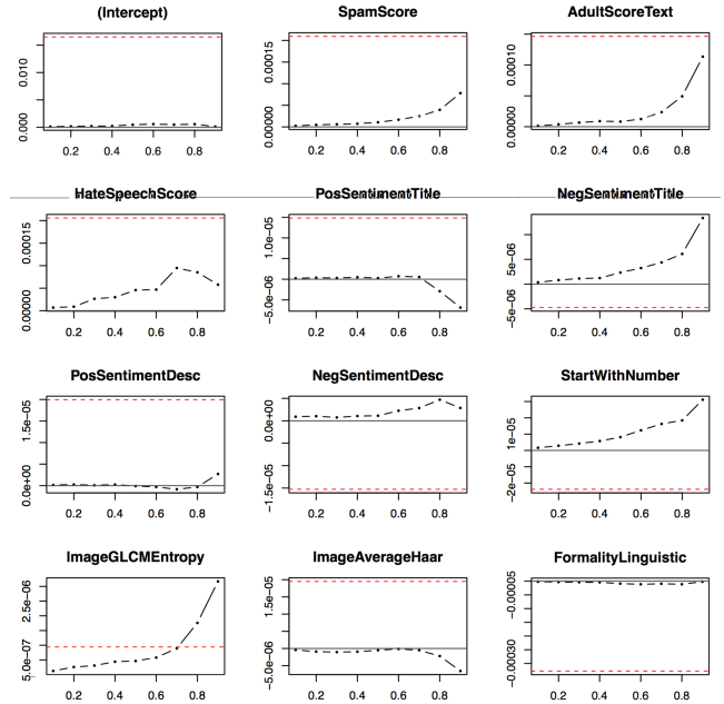
Figure 5: Quantile regression analysis of ad quality features to predict OFR.
