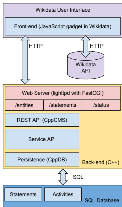
Figure 6: Primary Sources Tool architecture. The front-end (JavaScript) sends HTTP requests to the back-end (C++)
