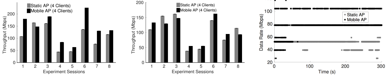
Figure 14: Throughput from real-time iMob with 4 clients: (a) Overall average throughput. (b) Average throughput when the AP is mobile, showing that AP mobility does not impose a performance penalty. (c) Data rate variation before and after stopping – the mobile AP’s rates are comparable to the Static until it stops, and higher thereafter.
