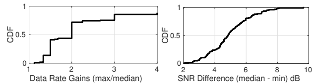
Figure 4: (a) CDF of (max/median) data rates in a box indicates gain at a client. (b) CDF of (median - min) SNR in a box indicates gain from avoiding interference.
