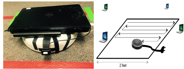
Figure 2: (a) A laptop and a webcam mounted on a Roomba to emulate a iMob AP. (b) Raster scan in a box while communicating to scattered client(s).
