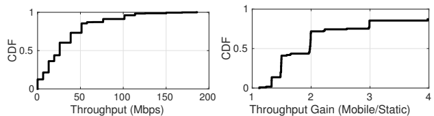
Figure 6: (a) CDF of throughput for each client during AP's mobility. (b) CDF of (max/median), i.e., the Oracle's gain over a randomly placed static AP.
