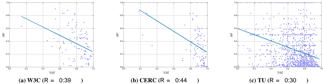
Figure 2: Scatter plot of the normalized entropy of distribution P(c|j|q) (2) returned by the log-linear model and per-query average precision for W3C, CERC and TU benchmarks. Pearson’s R and associated p -value (two-tailed paired permutation test: p < 0:01 ; p < 0:05 ; p < 0:1 ) are between parentheses. The depicted linear fit was obtained using an ordinary least squares regression.
