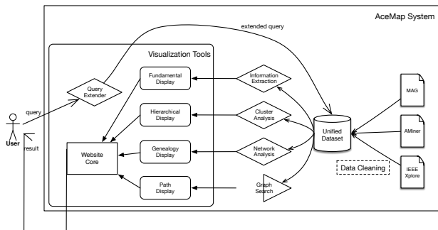
Figure 1: The Architecture of AceMap System.
