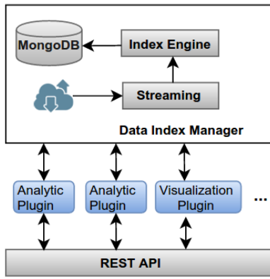
Figure 1: LODVader Architecture
