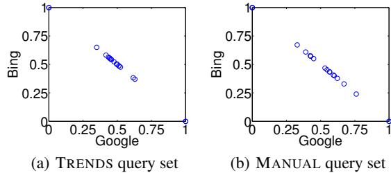
Figure 3: Visualization of TENSORCOMPARE for Google and Bing. Values on the x -axis correspond to the membership of Google to a cluster, and values on the y -axis correspond to the membership of Bing. Thus, an (x, y) point on this plot represents one of the clusters of TENSORCOMPARE. The closer the points are to the 45-degree line, the more similar are the two search engines.
