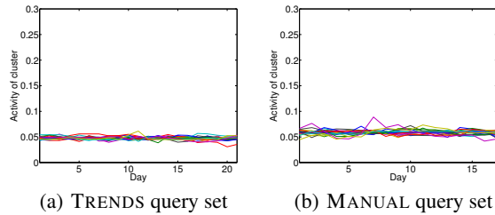
Figure 4: Temporal profile of latent clusters given by TENSORCOMPARE, for Google and Bing. The y -axis corresponds to the membership of the particular day to the cluster of interest. For both query sets, the temporal profile of all clusters is approximately constant over time. In particular, each value for TRENDS is \approx 1/21 and for MANUAL it is \approx 1/17 . As stated in Section 3.1, this indicates that both Bing and Google returned persistent results, at least during the duration of our experiment. Due to this uniformity, we overplot all clusters, without making any distinctions.
