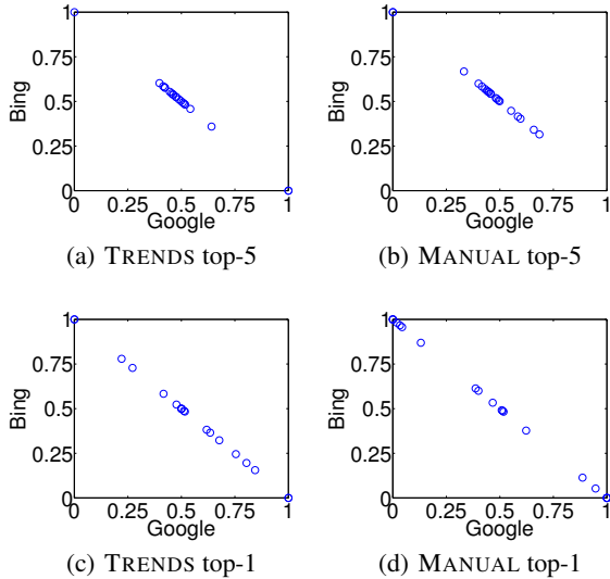
Figure 6: TENSORCOMPARE sensitivity
