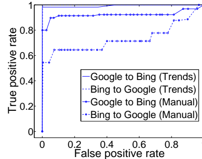
Figure 5: ROC curves produced by CrossLearnCompare (higher is better in terms of classification accuracy). If two search engines were completely mutually predictable, the ROC curve would be exactly on the (0, 0) - (0, 1) and (0, 1) - (1, 0) lines. Conversely, if two search engines were completely mutually unpredictable, the ROC curve would lie on the (0, 0) - (1, 0) and (1, 0) - (1, 1) lines. Finally, when the classifier is random, the curve would lie on the 45-degree line.
