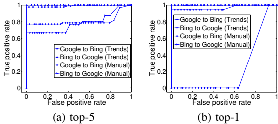
Figure 7: CROSSLERNCOMPARE sensitivity
