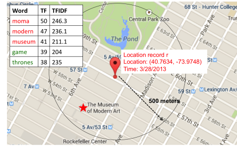
Figure 3: An example illustrating the problem of frequency based methods. The true user’s intention of this location record is to attend the Game of Thrones event. But since MOMA is a more popular venue nearby, frequency-based methods will incorrectly use words “moma” and “modern” for annotation.
