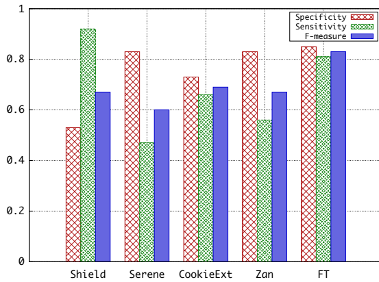
Figure 2: Performance evaluation
