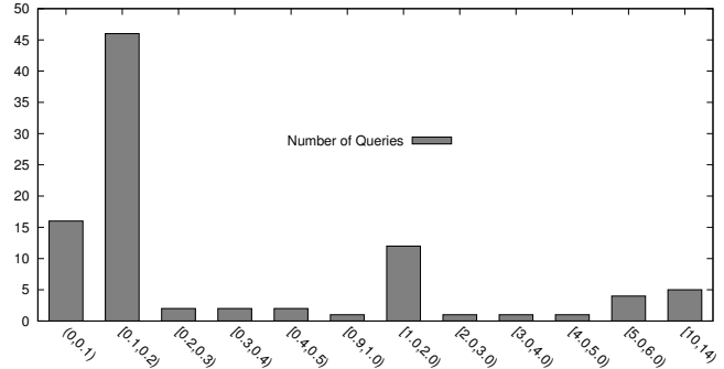
Figure 6: Synthetic UOBM queries. X axis is \frac{|\text{UB} \setminus \text{LB}|}{|\text{LB}|} ; Y axis is the number of queries falling in each interval on the X axis.
