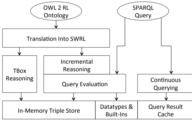
Figure 2: Reasoner’s Architecture
