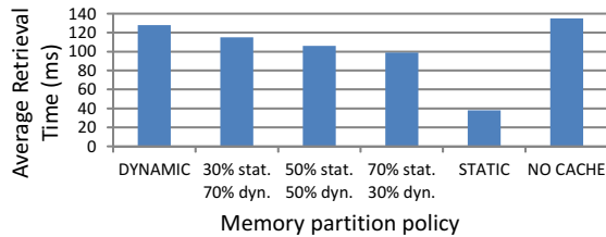
Figure 5: Average response time of various caching policies.
