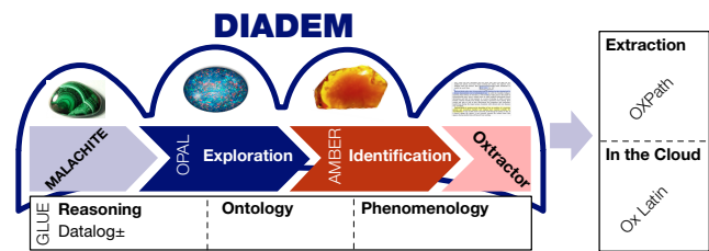
Figure 3: DIADEM Overview
