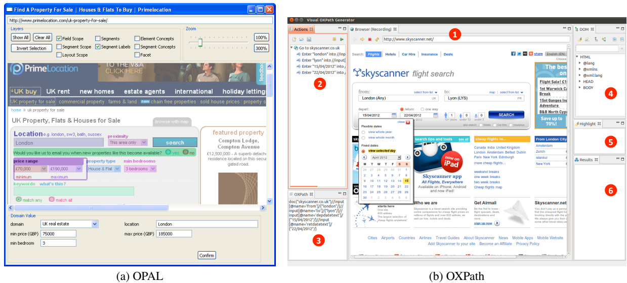
Figure 6: Demonstration UIs
