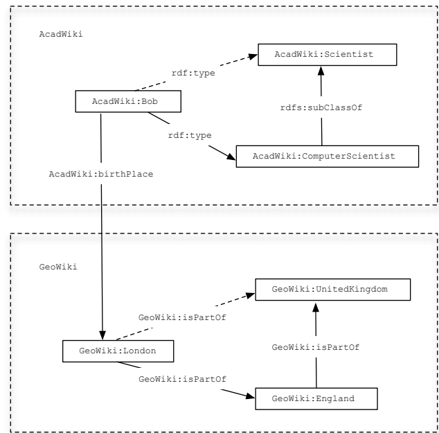
Figure 1: Extract of the RDF graphs from AcadWiki and GeoWiki
