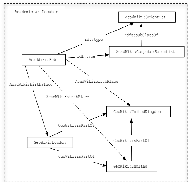
Figure 2: The new inferences made by the federated application shown by the dashed arrows
