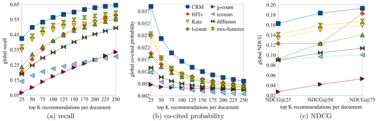
Figure 5: Compare performances for global recommendation.
