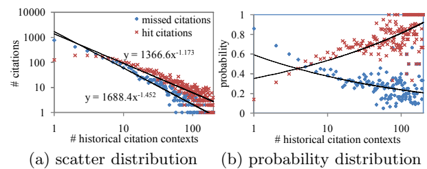
Figure 7: Correlation between count/probability of missed/hit citations and their number of historical in-link citation contexts.
