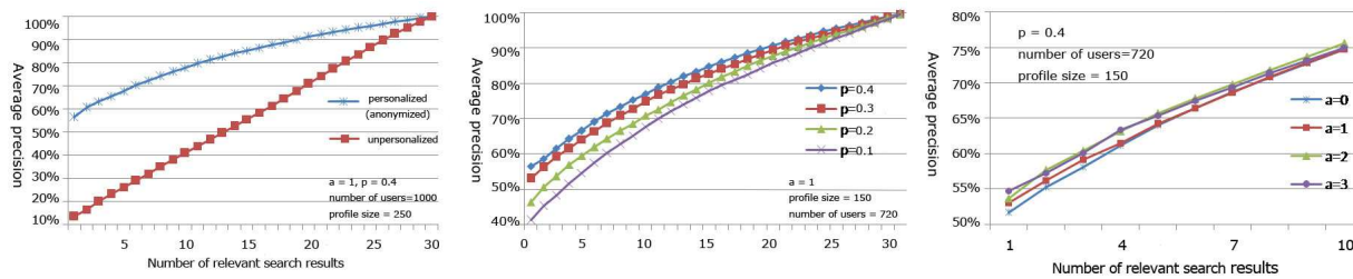
Figure 1: Search precision using anonymized user profiles
