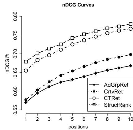
Figure 4: NDCG Curves.
