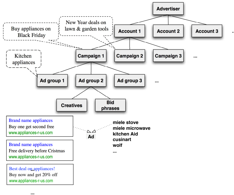
Figure 1: Schema of an ad database
