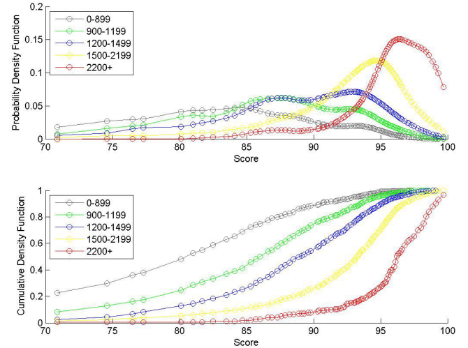
Figure 5: Distribution of Software Design Review Scores Clustered By Coder Rating
