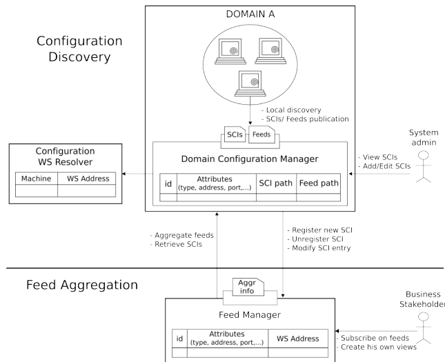
Figure 4. Configuration Management Architecture
