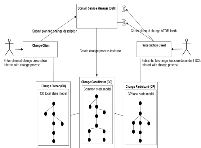
Figure 7: Change 2.0 Architecture Overview
