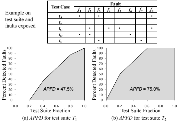
Figure 1. Example illustrating the APFD measure.
