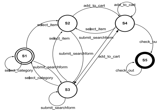
Figure 2: Process Automaton Example
