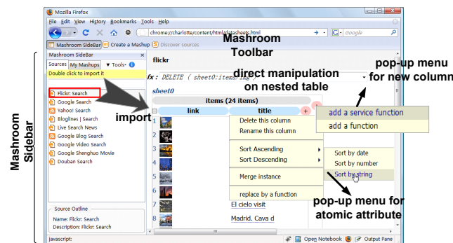
Figure 4. The Interface of Mashroom
