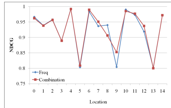
Figure 10. NDCG of Freq and Combination
