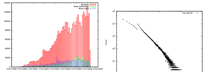
(a) Numbers of new users, new bookmarks, and new reviews per month.
