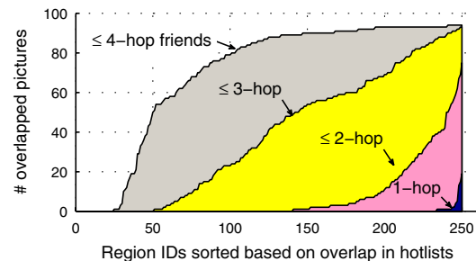
Figure 3: Resemblance in local and global hotlists
