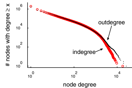
Figure 2: Node degree distribution
