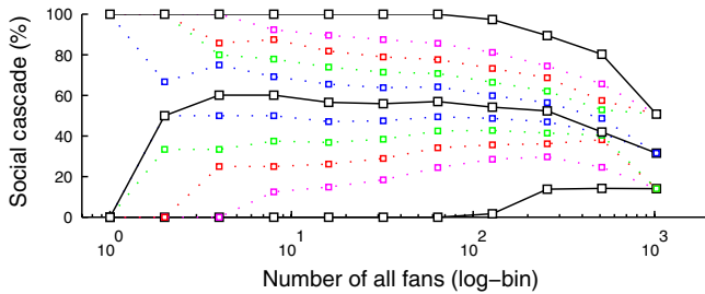
Figure 6: Probability of information flow through social links across picture popularity: Plot shows every 10th percentile probabilities including minimum, median, and maximum.
