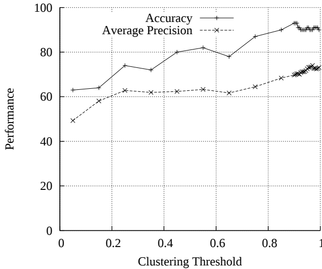
Figure 3: Performance of the proposed method against the clustering threshold ( \theta )
