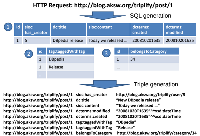
Figure 4: Triple generation from database views. The numbered query result relations correspond to the queries defined for the post URL pattern in the WordPress example configuration in Figure 3.
