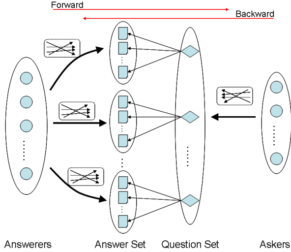
Figure 2: |Q| coupled bipartite graphs connecting with user-question bipartite graph.
