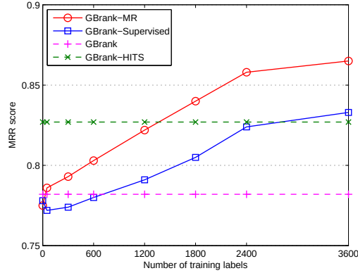
Figure 6: MRR of GBrank, GRank-HITS, GBrank-MR, and GBrank-Supervised for varying fraction of training labels used in CQA-MR
