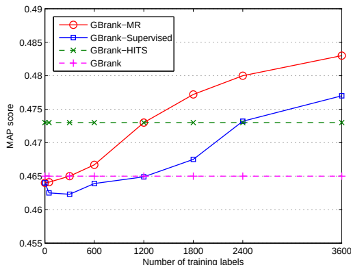
Figure 7: MAP of GBrank, GRank-HITS, GBrank-MR, GBrank-Supervised for varying fraction of training labels used in CQA-MR
