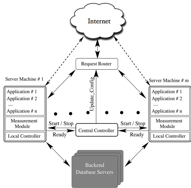
Figure 1: General architecture of a hosting platform.
