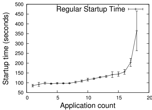
Figure 5: Application startup time vs. the number of pre-existing idle applications.
