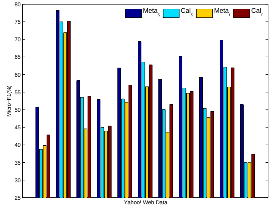
Figure 3: Meta-Models with Calibration
