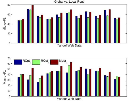
Figure 2: Meta c vs. RCut
