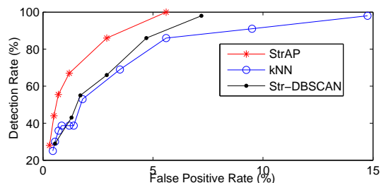
Fig.2. ROC curves with Str-DBSCAN, StrAP and k-NN
