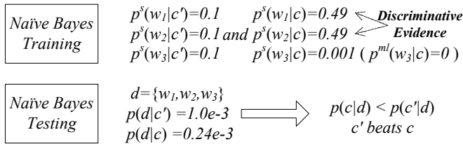
Figure 2: Illustration of discriminative evidence cancelation problem where we assumed p(c) = p(c') . Besides, there is p(c|d) = p(d|c)p(c)/p(d)
