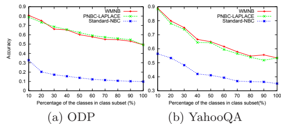
Figure 3: Standard NB, WMNB and PNBC-Laplace with different number of classes
