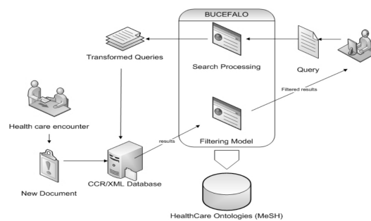
Figure 1: Tool Architecture
