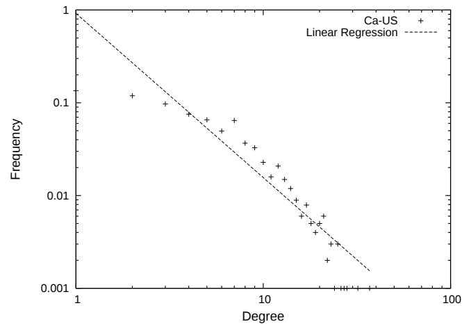
Figure 3: Degree Distribution for Ca-US Network (Log-Log Scale)
