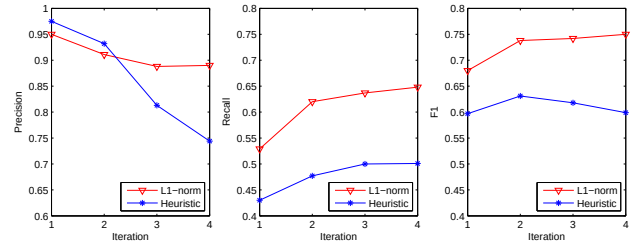
Figure 4: The performance (precision, recall, and F1) of the two StatSnowball systems with joint inference during the iteration.
