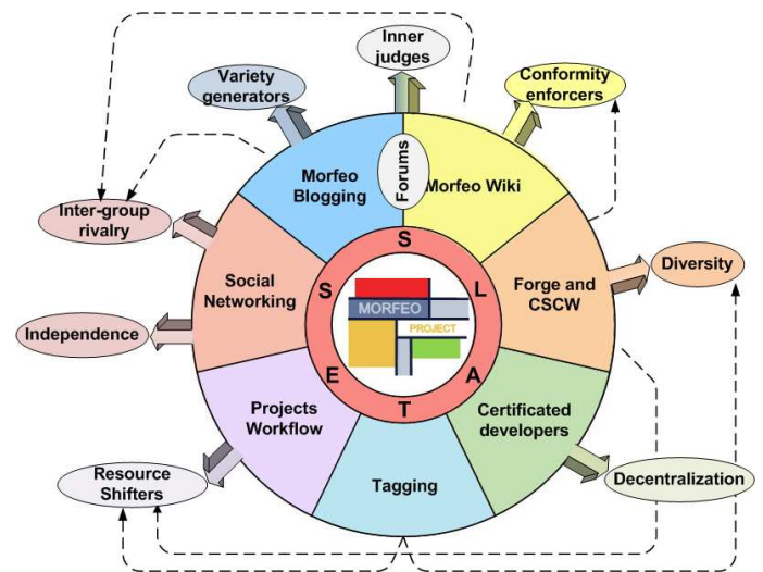
Figure 1: Morfeo framework
