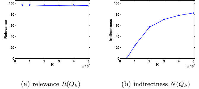
Figure 2: Plots for evaluation metrics for Health
