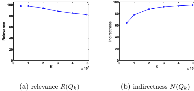
Figure 1: Plots for evaluation metrics for Shoes
