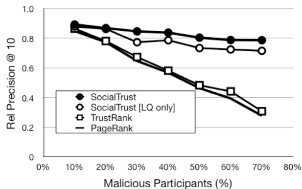
Figure 1: Comparing trust models
