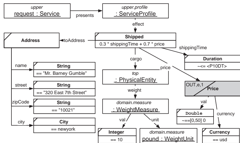
Figure 1: Simplified DSD shipping request
