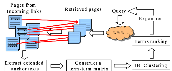
Figure 1: The topic-oriented query expansion model
