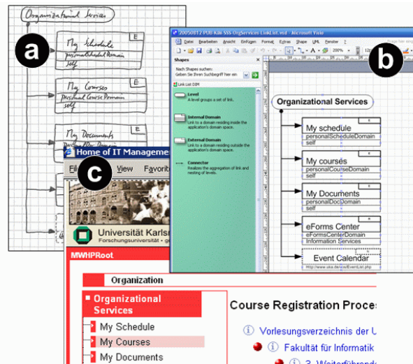
Figure 2: Application of the Linklist DSL: (a) pen and paper drafted DIM, (b) MS Visio DIM, (c) applied and executed DSL program within a portal based on the WLS framework.
