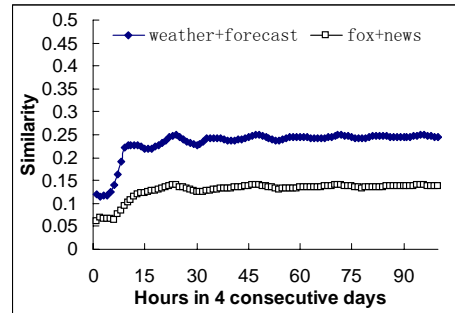
Figure 10: Query similarity with incremented approach
