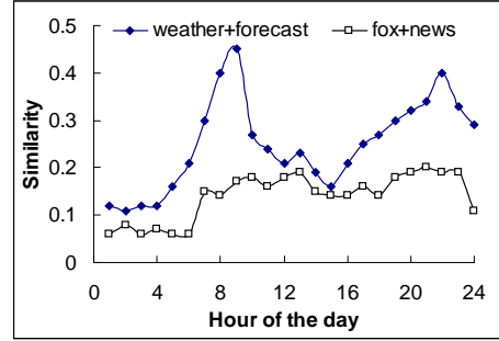
Figure 9: Hourly-based time dependent query similarity model
