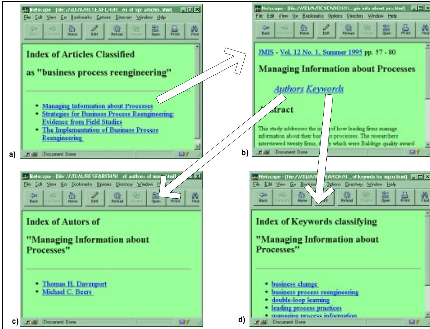
Figure 3: Pure RMM is limited in its functionality. The user would have to navigate from page a), which contains only the titles of the articles classified under “business process reengineering” to screens b) and c) to find out the names of the authors of that article; and to d) in order to find other keywords classifying the same article. The extensions to RMM we present here enable richer designs that are more natural to the user.
